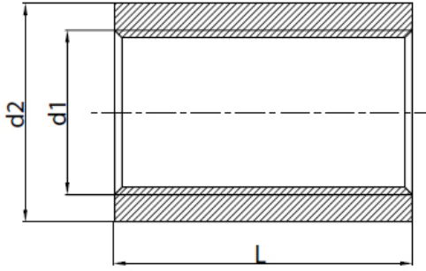
TAM MANŞON FULL COUPLING
